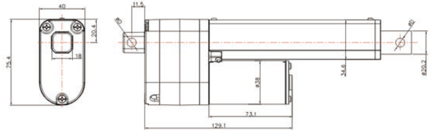
Optional Trunnion Mounting Position
